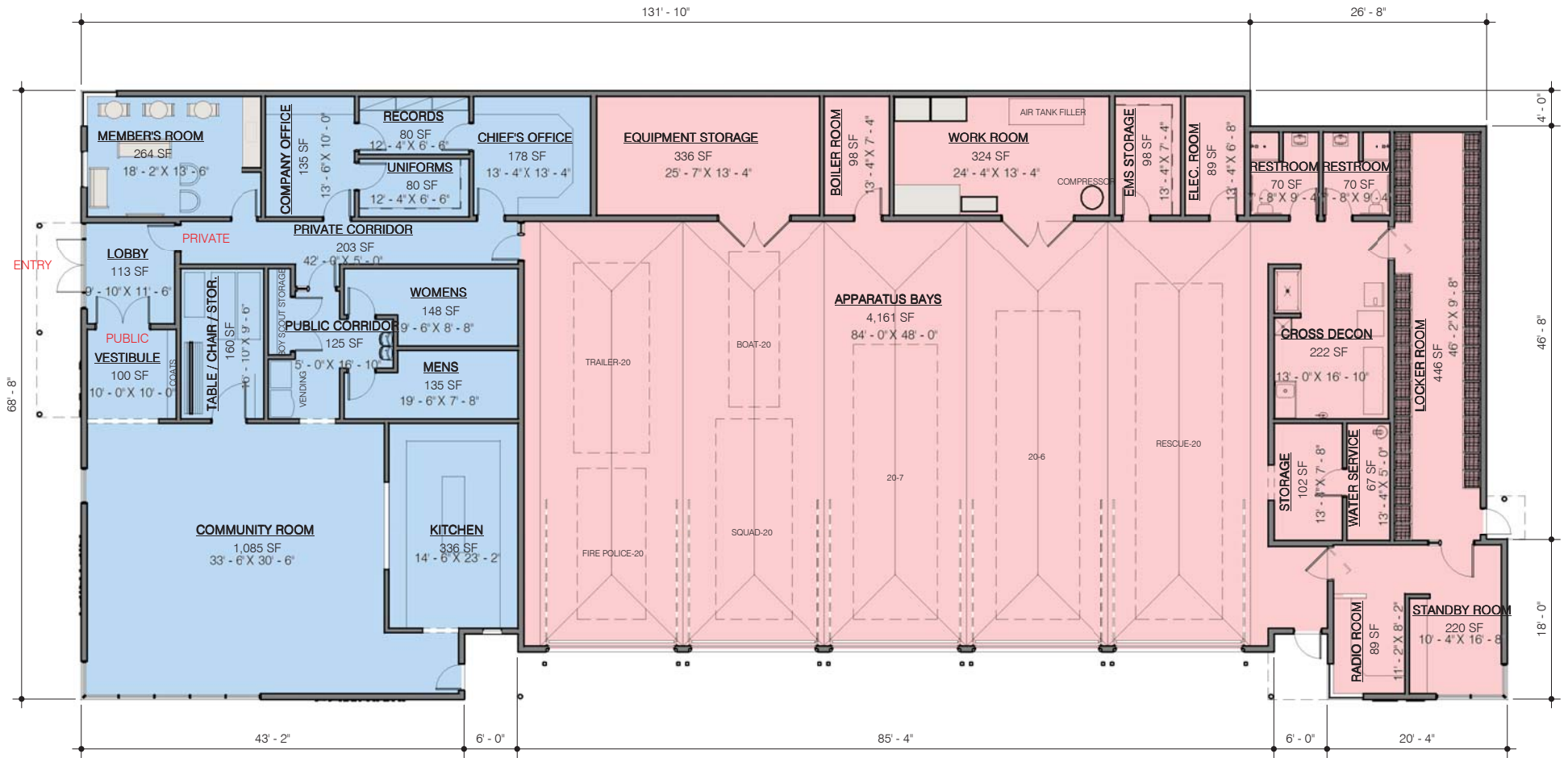
REVISED FLOOR PLAN DATED AUGUST 27, 2020 10, 276 SF
